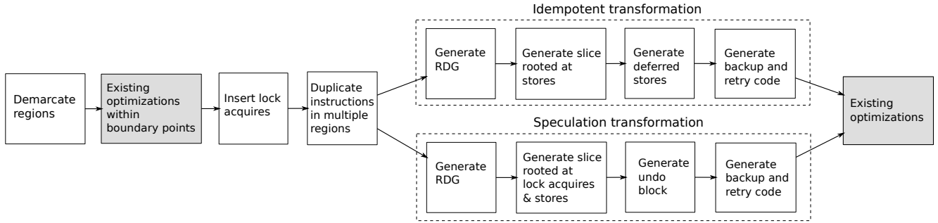
Figure 1. The transformations performed by an EnfoRSer-enabled optimizing compiler. Boxes shaded gray show existing compiler optimizations. Dashed boxes indicate transformations performed once on each region.
