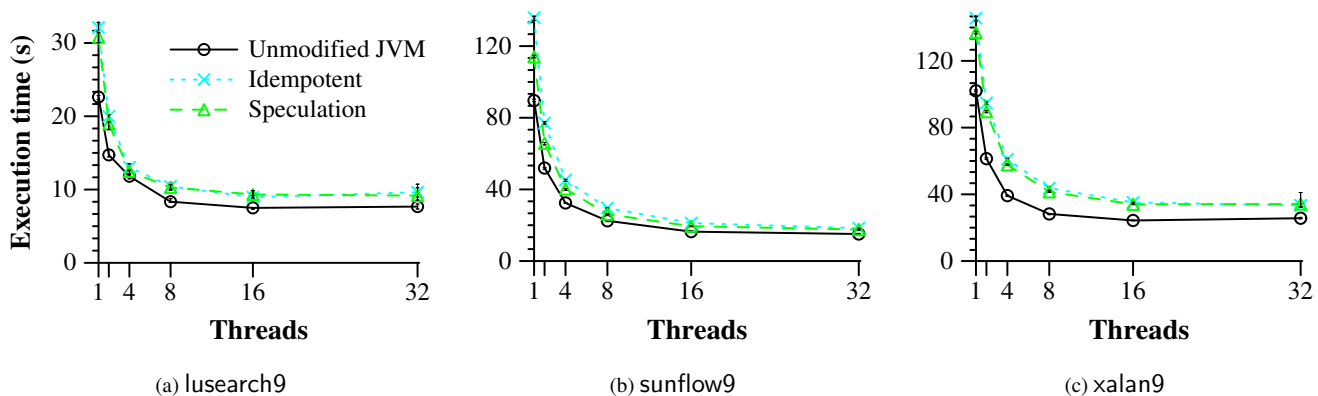
Figure 8. Scalability of EnfoRSer’s approaches, compared with the unmodified JVM, across 1–32 application threads.
