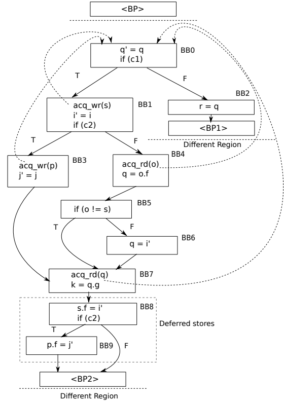
Figure 4. Region from Figure 2 after idempotent transformation.
