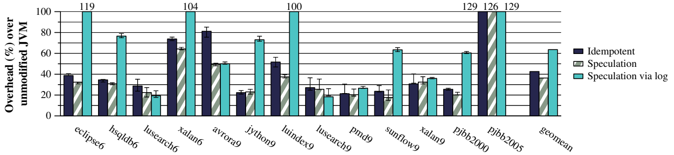
Figure 6. Run-time overhead over an unmodified JVM of providing SBRS with EnfoRSer’s two atomicity transformations and speculation that uses a log to simulate a stripped-down version of STM.
