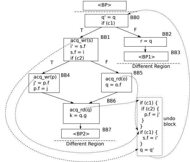
Figure 5. Region from Figure 2 after speculation transformation.
