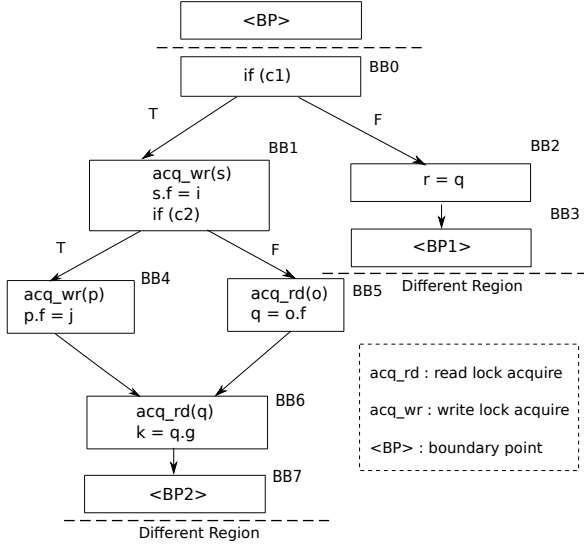
Figure 2. A region instrumented with lock acquire operations.
